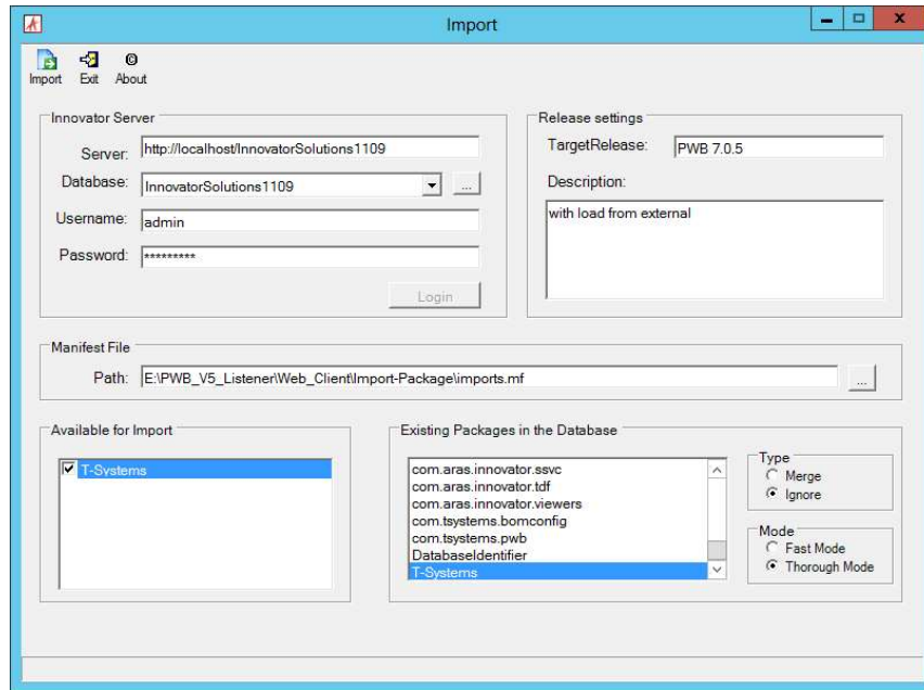
Picture 44: Import utility
